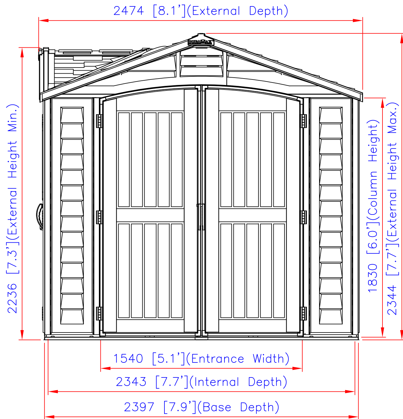
Side View
